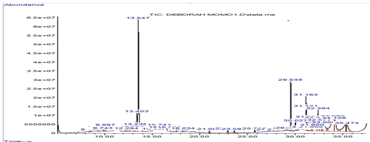
Figure 2: GC-MS spectrum of ethyl acetate fraction of OL
